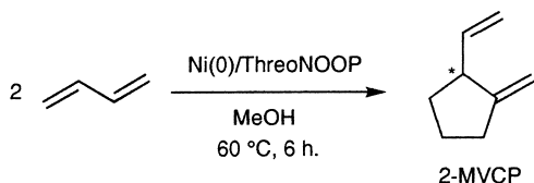
Scheme 4. Cyclic dimerization of butadiene.
