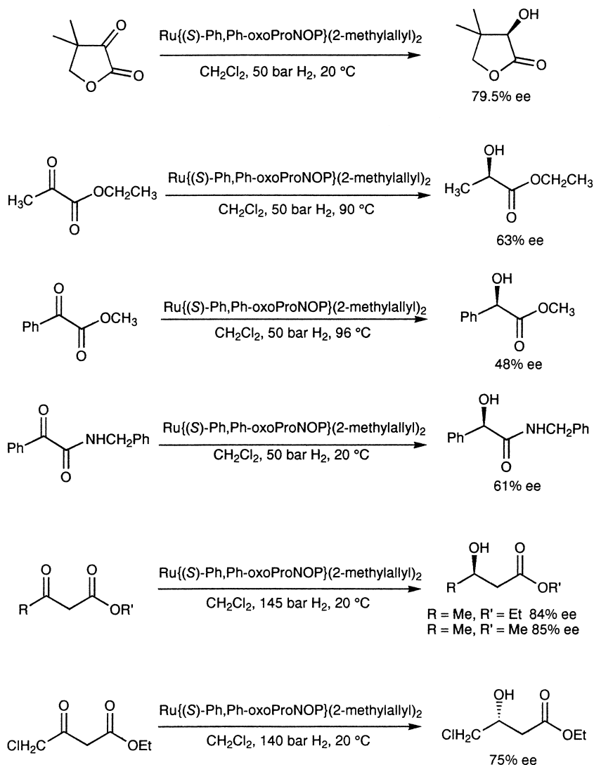
Scheme 29. Ruthenium catalysed asymmetric hydrogenation of functionalized ketones.
