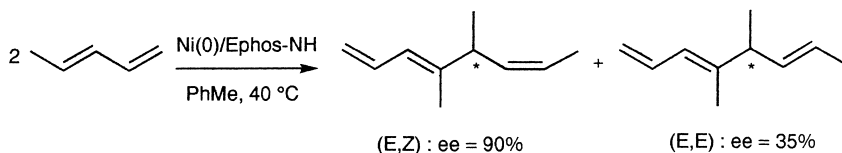
Scheme 6. Nickel catalysed dimerization of piperylene.
