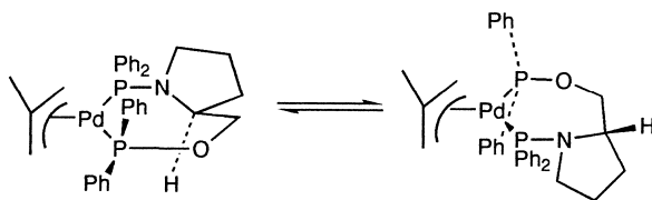
Scheme 14. Diastereomeric palladium {ProNOP} complexes.
