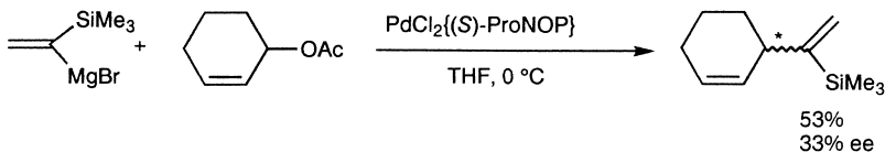
Scheme 16. Palladium catalysed allylic substitution.
